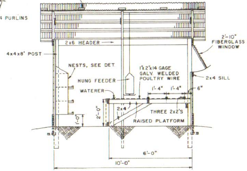
CROSS SECTION
